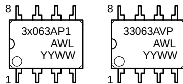
PDIP-8 P, P1 SUFFIX CASE 626
