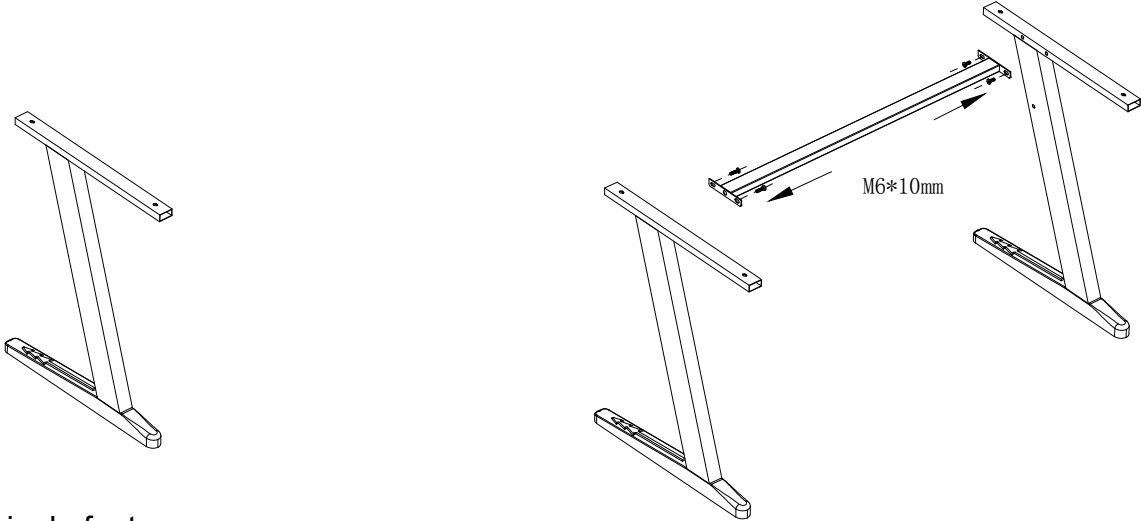
1.Put the single foot 2.The single foot is connected with the tie rod with screws
