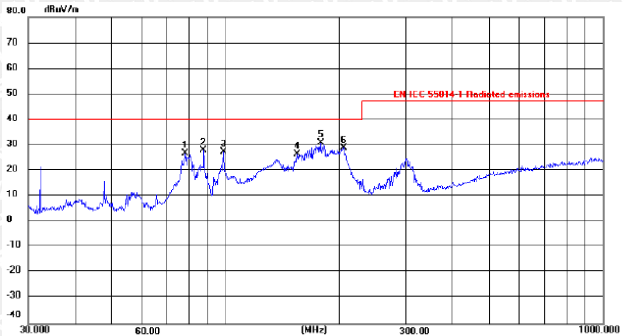
Figure 3: Test Curve of Radiated Emission in the frequency range of 30-1000MHz, Horizontal
