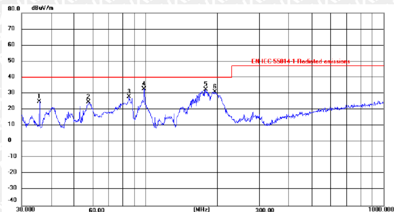
Figure 4: Test Curve of Radiated Emission in the frequency range of 30-1000MHz, Vertical
