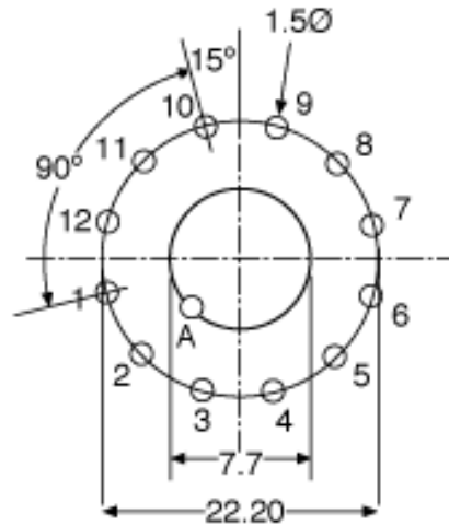
PIN LAYOUT (Top View)
