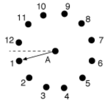
SWITCHING DIAGRAM (Top View)
