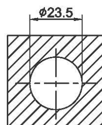
PANEL APERTURE
