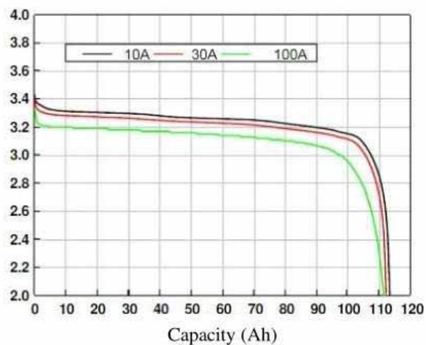
Curve of cell discharge
