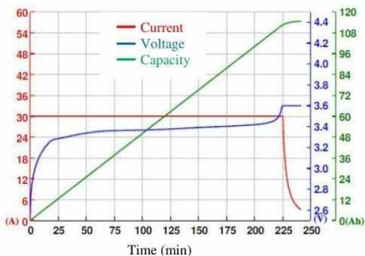
Curve of cell charging
