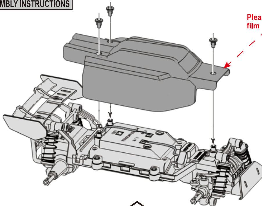
Bodyshell * 1
