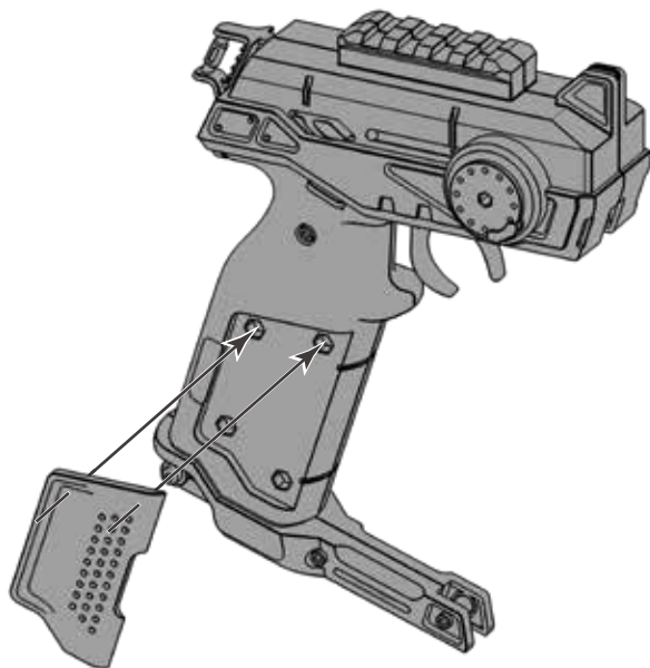
Handle Patch * 1
