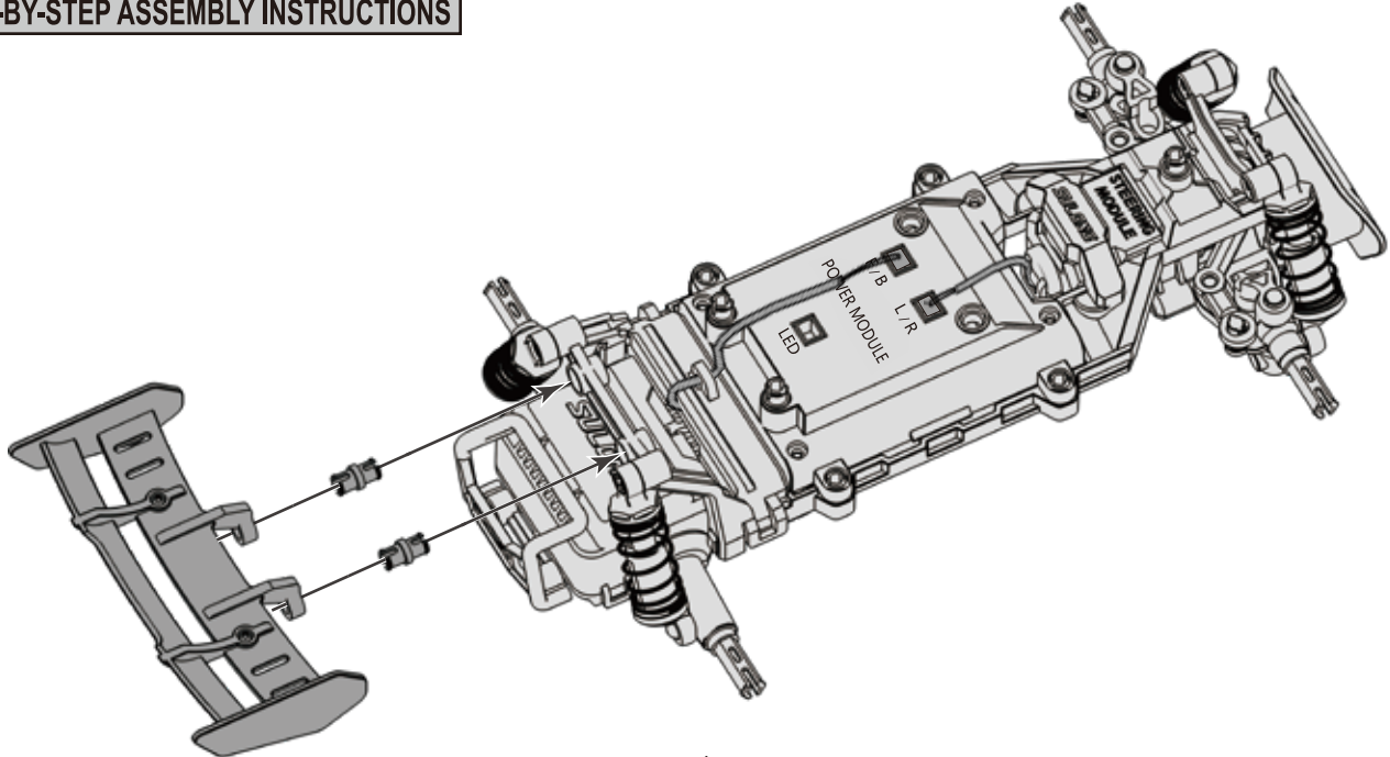
Latch C1 * 2
