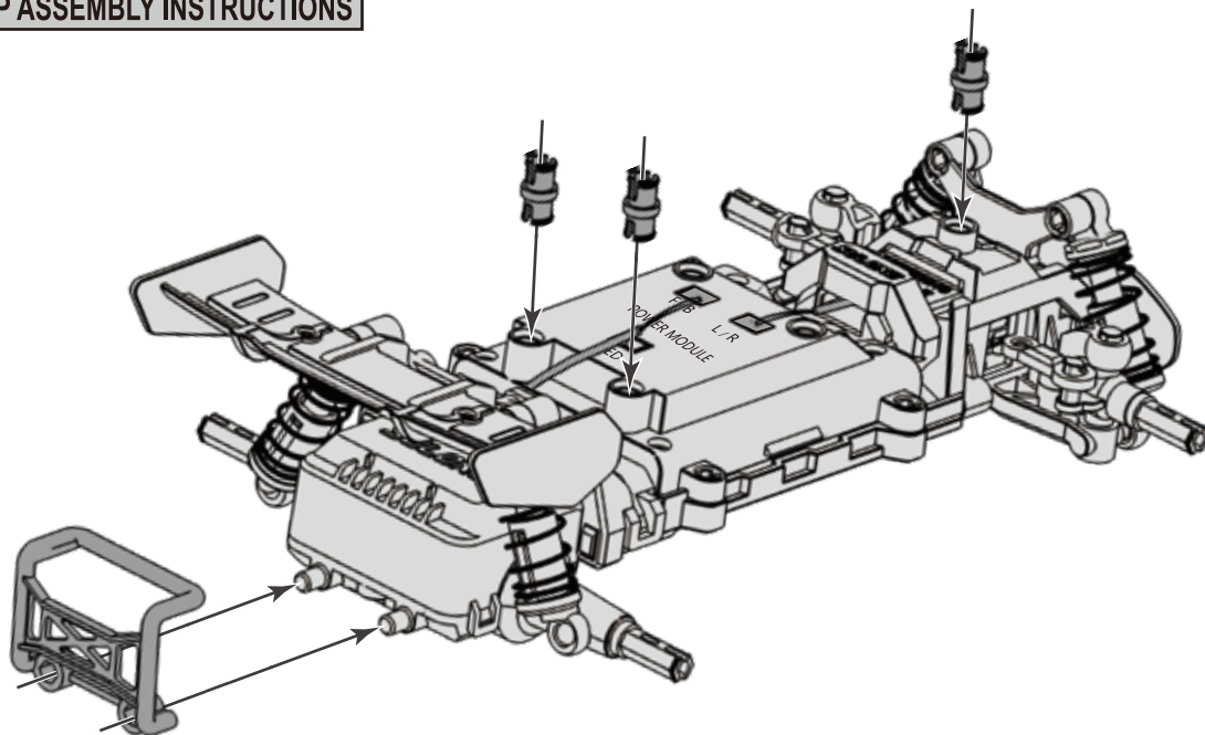
Latch C1 * 3
