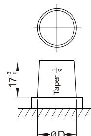
Standard Terminal (mm)
